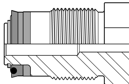
Jetstream Pump Discharge (All 40K UNx Fluid Ends)
