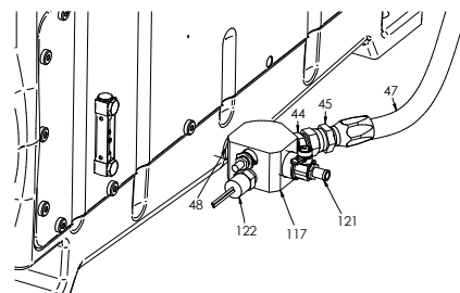
REAR PUMP OIL DRAIN ASSY
