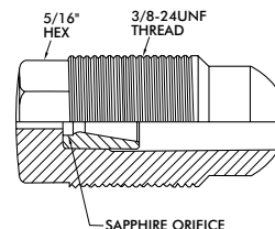
40K 4" J-FORCE, UNIVERSAL WITH FRONT NOZZLE
