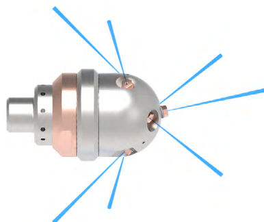
UNIVERSAL NOZZLE ANGLES
